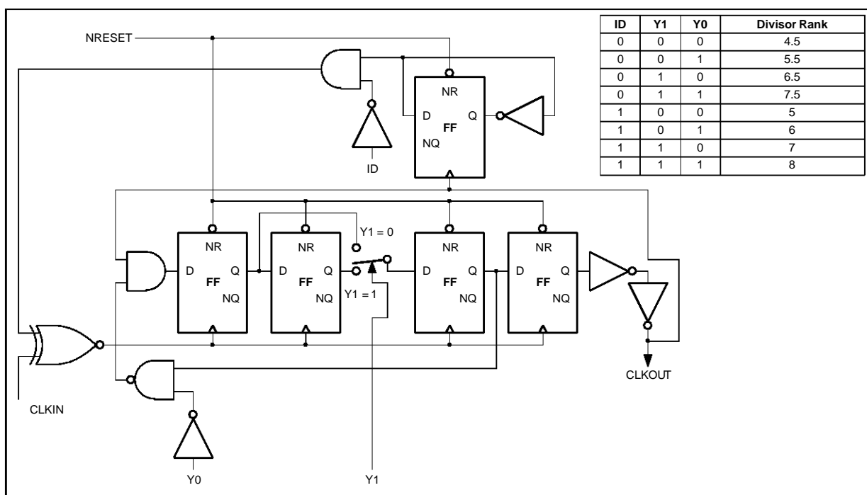
Figure 19 : Programmable Divider by 4.5, 5.5, 6.5, 7.5, 8
