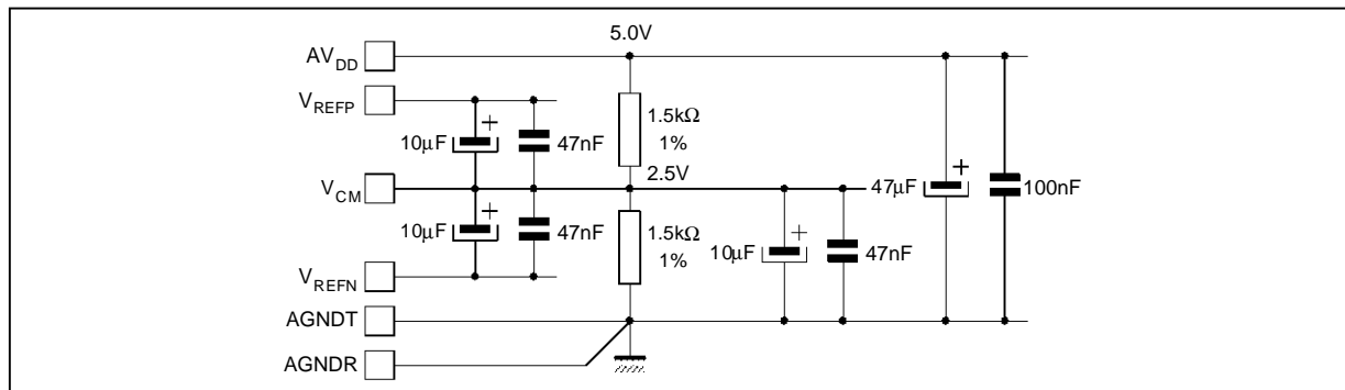
Figure 17 : Voltage Decoupling
