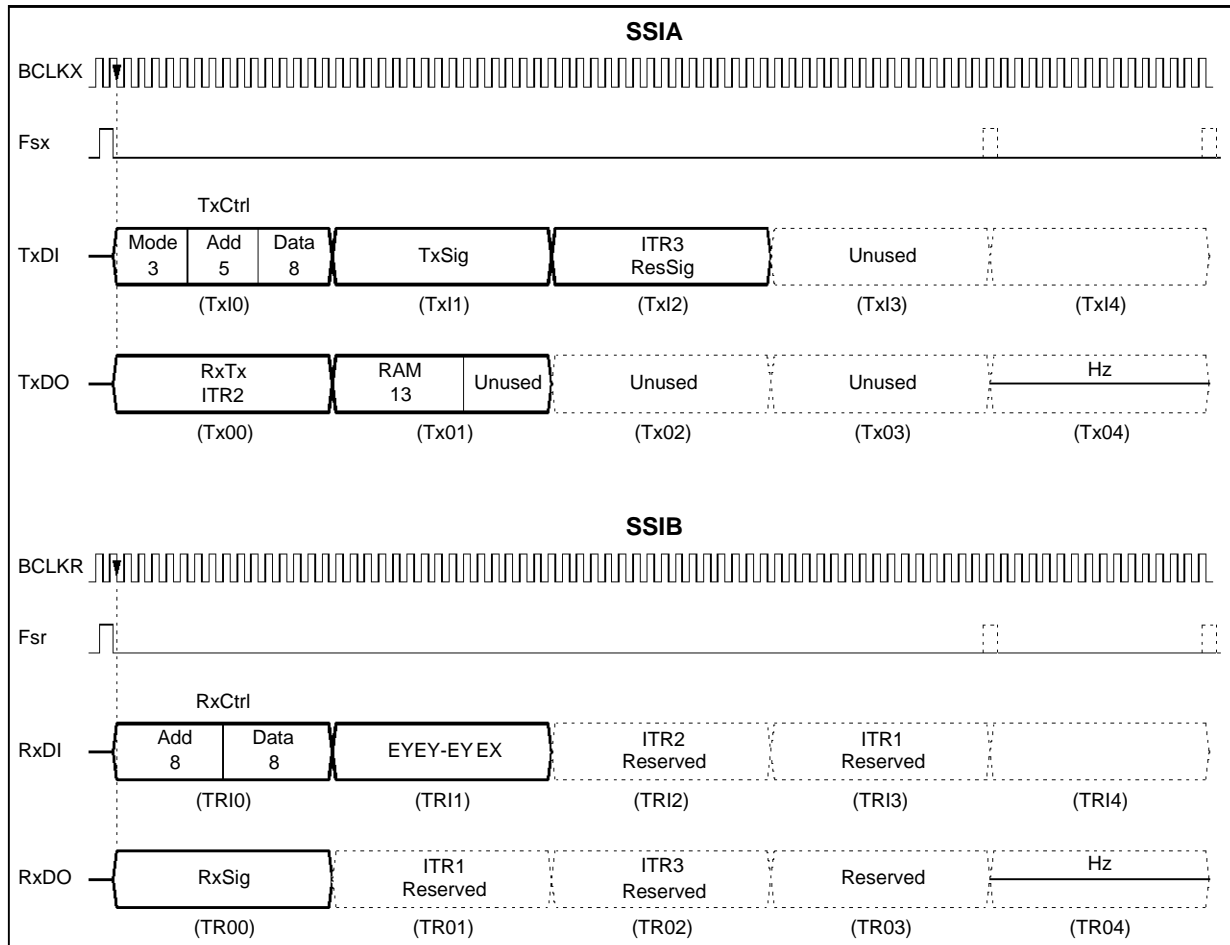
Figure 6 : Serial Channel Timing. Dual Port Mode
