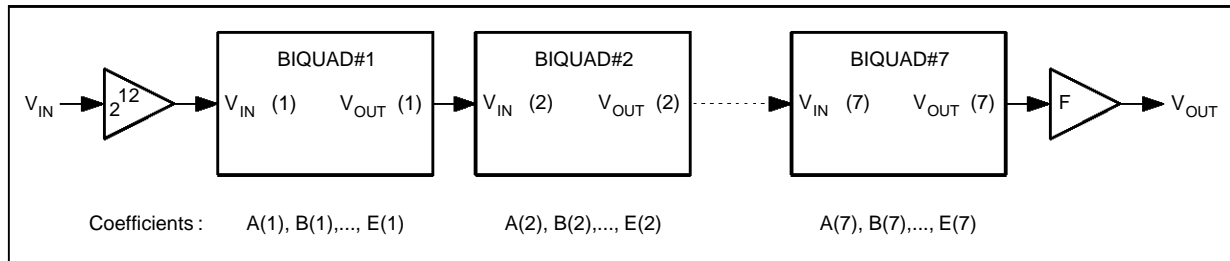
Figure A1 : IIR Filter Diagram
